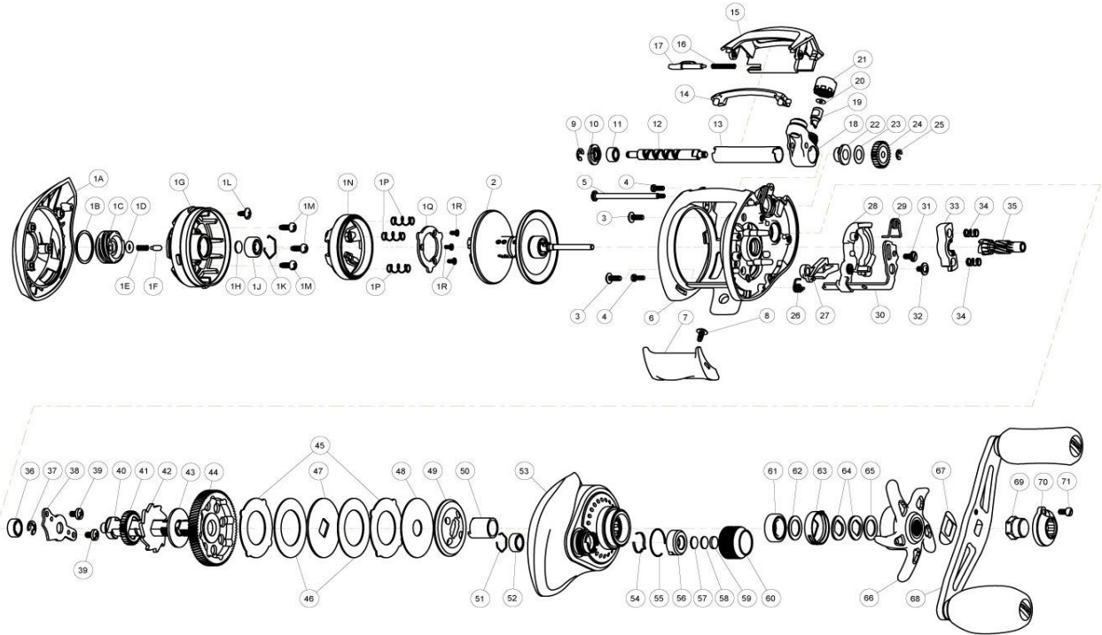
Smoke SHD200PPT Baitcast Reel Part List
